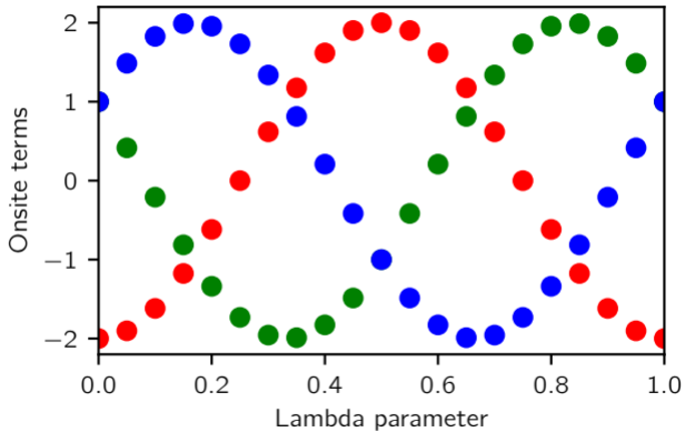
Onsite energy for all three orbitals
