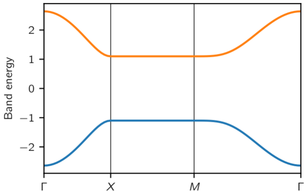
Bandstructure for buckled rectangular layer
