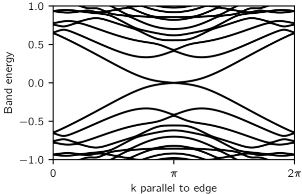
Graphene arbitrary surface band structure
