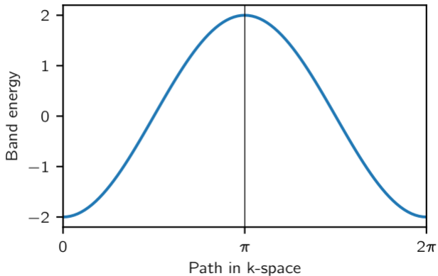
1D chain band structure
