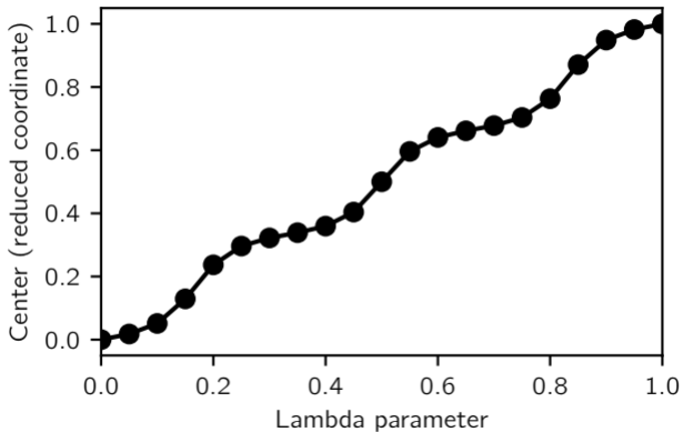
Center of Wannier function
