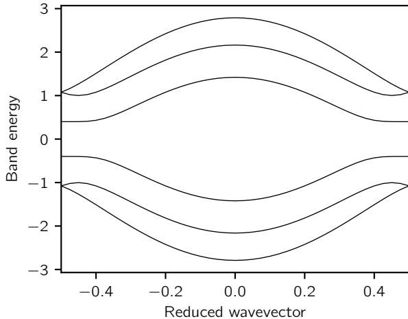
Band structure - modified
