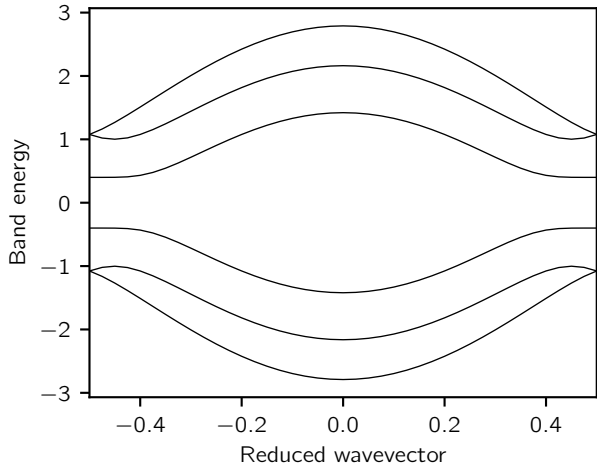
Band structure - original
