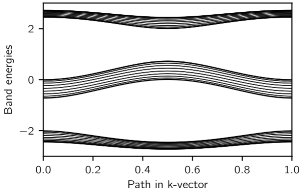
Band structure
