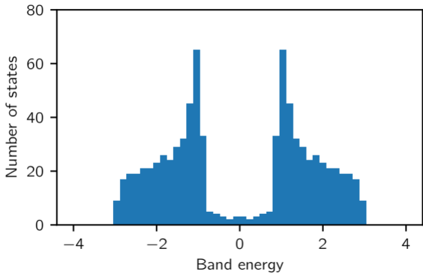
Finite Haldane model without PBC
