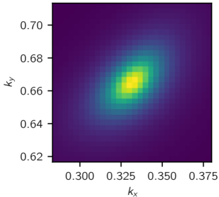
Berry curvature near Dirac cone
