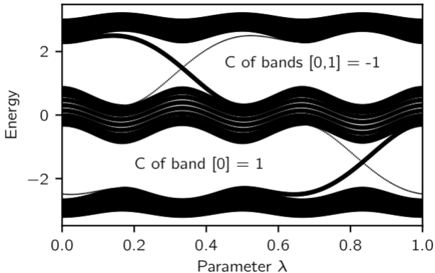
Eigenenergies for finite chain of 3-site-model
