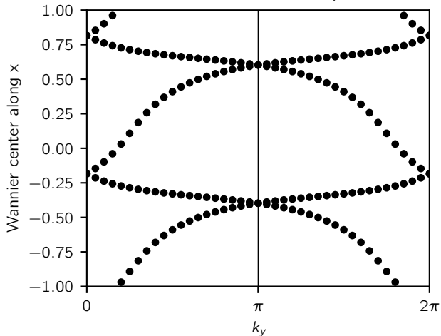
1D Wannier centers: odd phase
