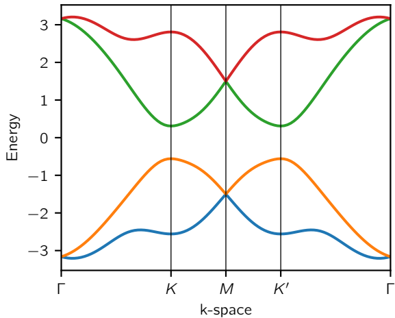
Kane-Mele: odd phase
